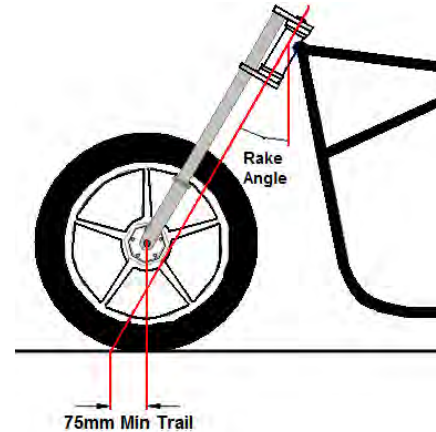
Motorbike Trail
